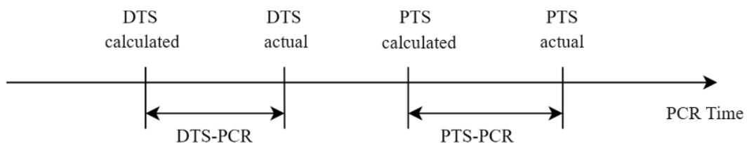
Figure 25 – Illustration of DTS-PCR and PTS-PCR
